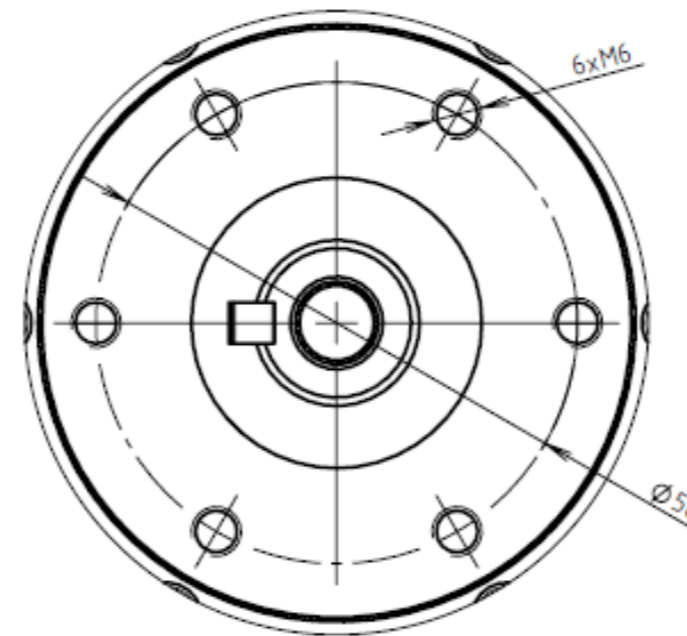
PROPELLER BOLTS PATTERN SCALE 1:1
