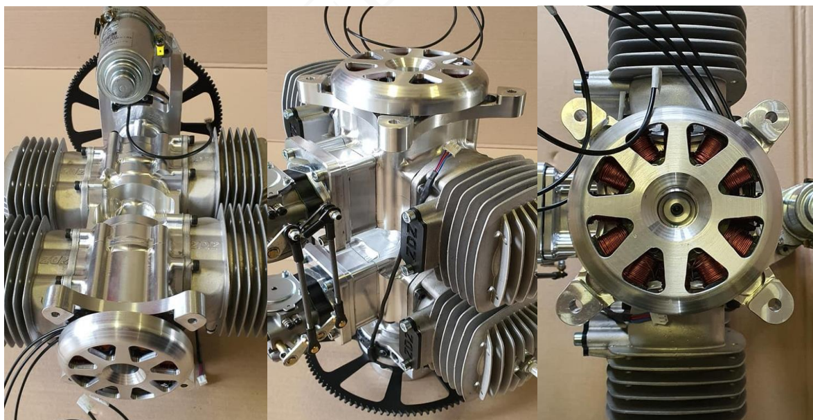
Picture 3 Installation example on ZDZ 390B4-JS
