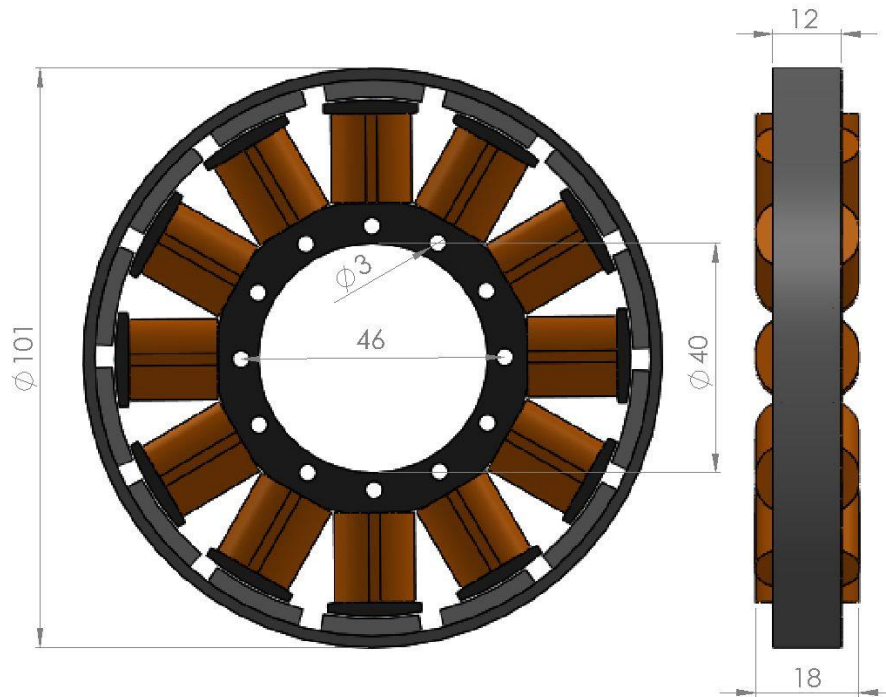
Picture 2 Basic dimensions of ZDZ GEN 101/9/12
